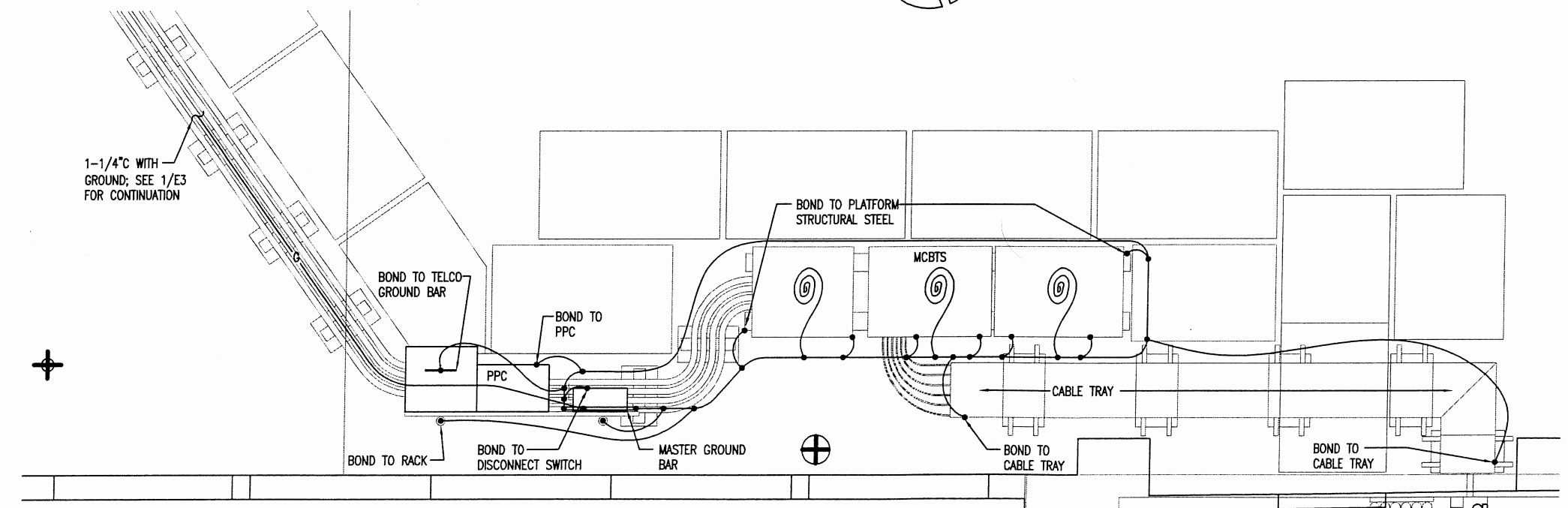
1 ENLARGED PLATFORM ELECTRICAL PLAN SCALE: 1"=20'-0"
