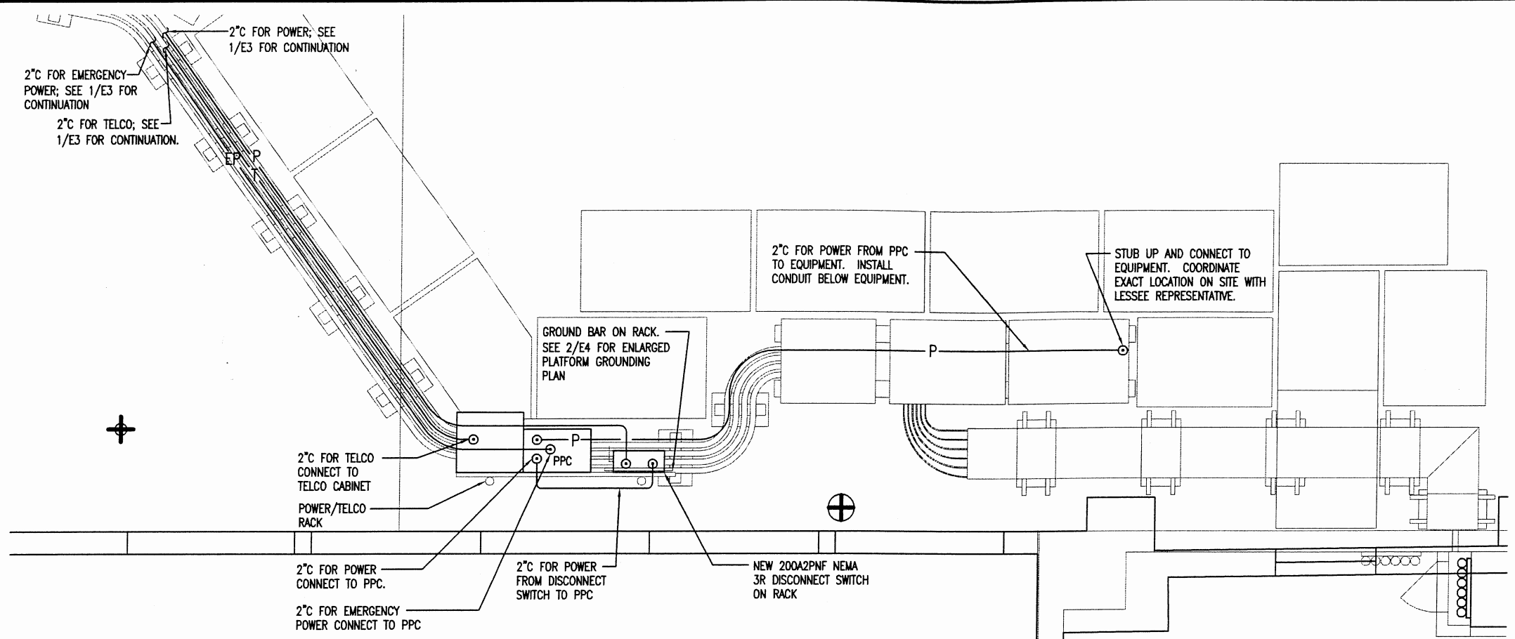
1 ENLARGED PLATFORM ELECTRICAL PLAN SCALE: 1"=20'-0"
