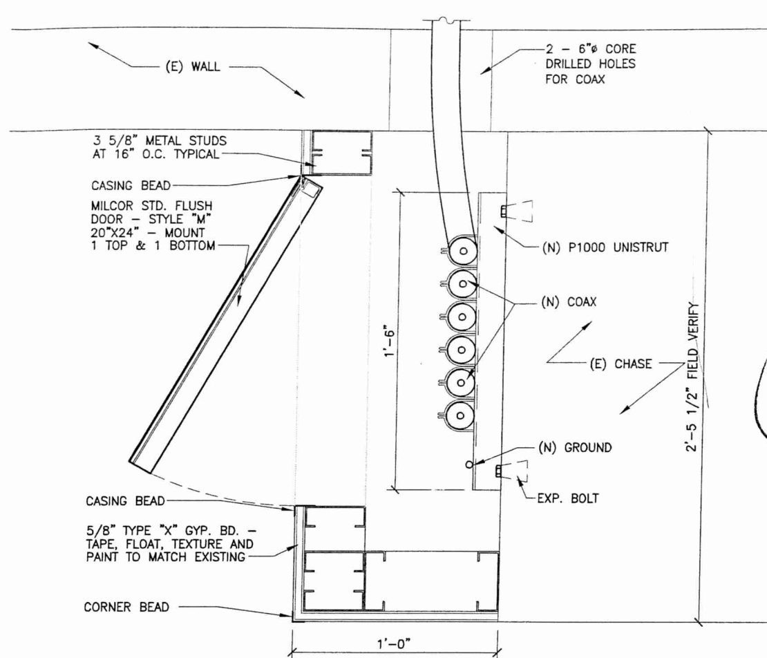
2 PLAN AT COAX CHASE SCALE: 1 1/2" = 1'-0"
