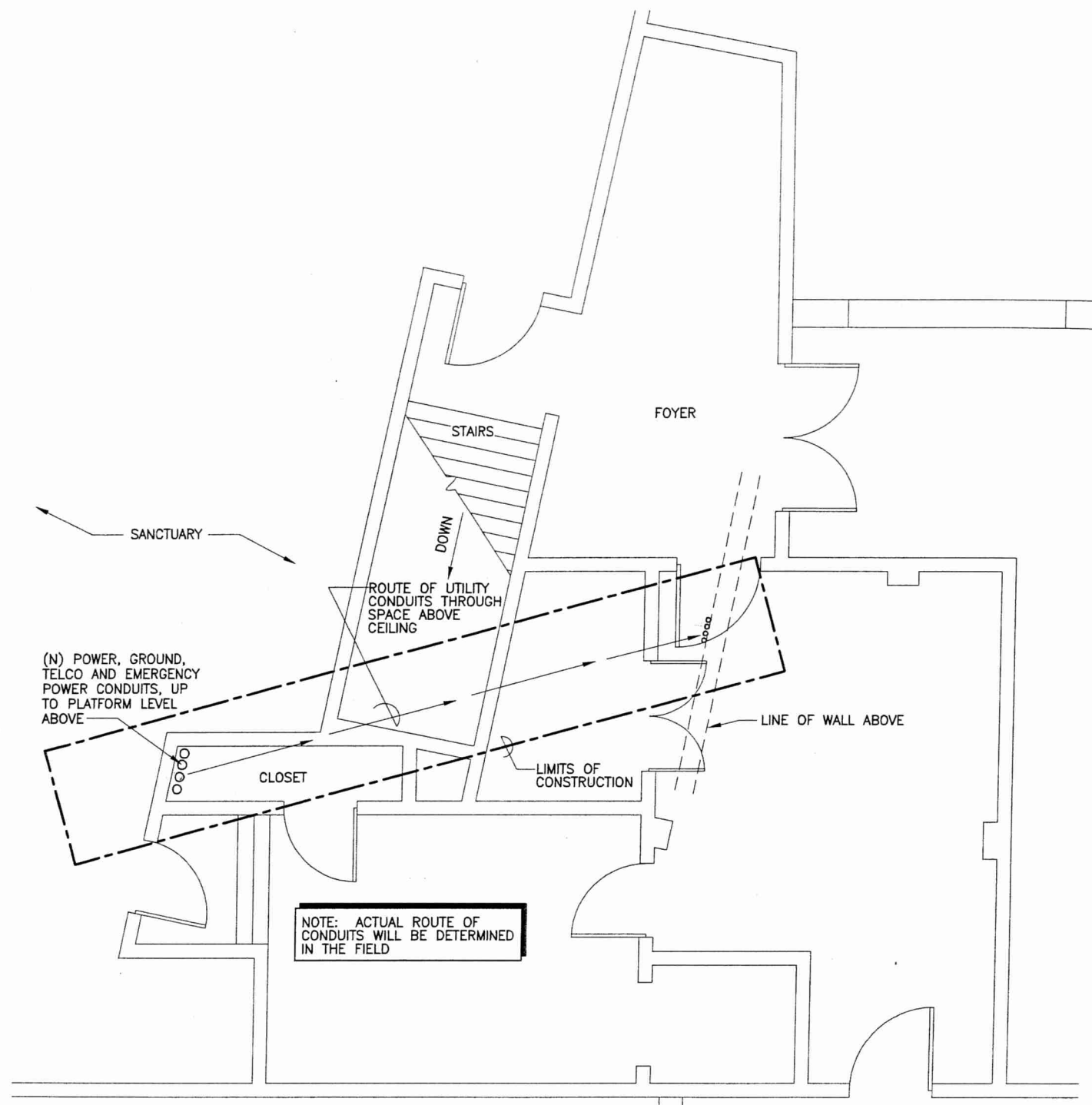
1 1ST FLOOR PLAN SCALE: 3/16" = 1'-0"
