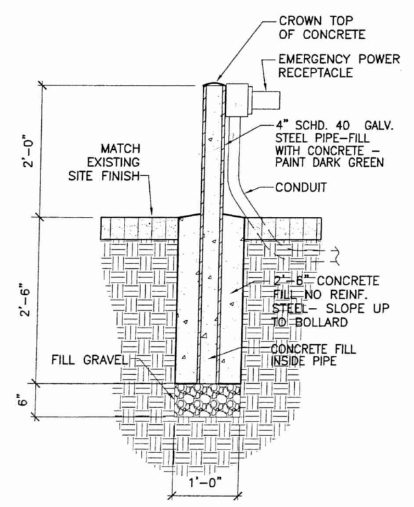
3 EMERGENCY POWER RECEPTACLE MOUNTING SCALE: 1/2" = 1'-0"
